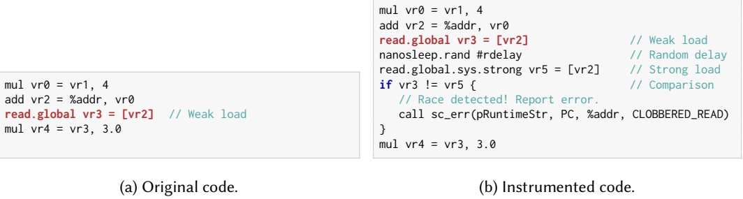
Fig. 1. SuperCollider instrumentation for weak loads. (a) Original code. (b) Instrumented code with delay and strong load for race detection. We extend this approach to similarly handle writes and asynchronous memory copies.
