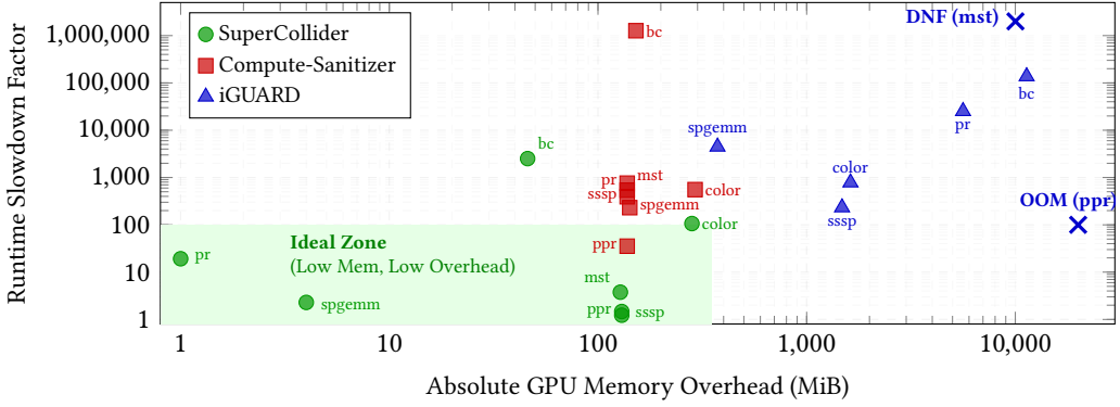
Fig. 11. Performance vs. Memory Overhead on Gunrock. The y-axis shows the runtime slowdown, where native execution is 1. The x-axis shows the additional GPU memory required (MiB). SuperCollider clusters in the low-overhead ideal zone, whereas Compute Sanitizer incurs large runtime penalties, and iGUARD experiences significant memory bloat (leading to OOM/DNF failures on large workloads).
